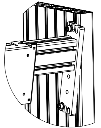
DETAIL B SCALE 1 : 4
