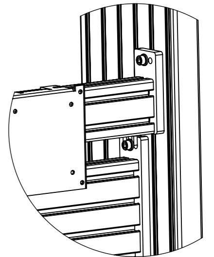
DETAIL A SCALE 1 : 4
