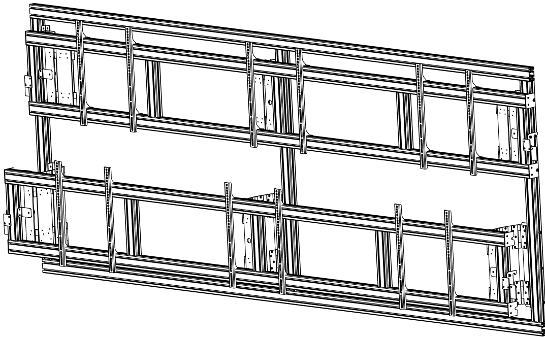
3x2x46" Video Wall shown with pop out mechanism
