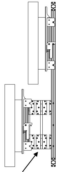
Side view of pop out mechanism showing access to rear of screen for service and maintenance
